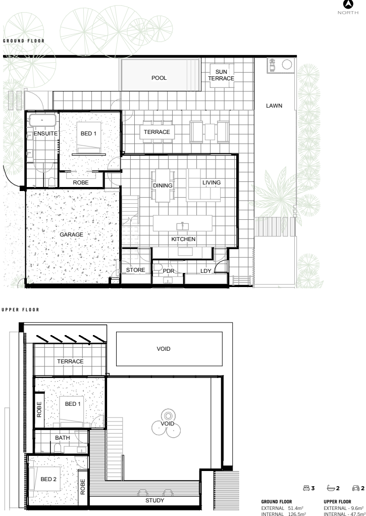
TOWNHOME TWO B
